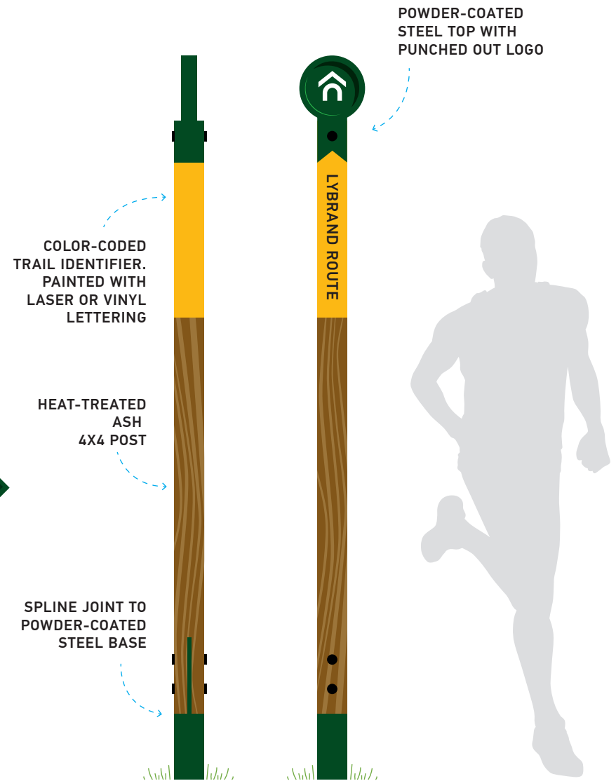
BASIC TRAIL SIGN
