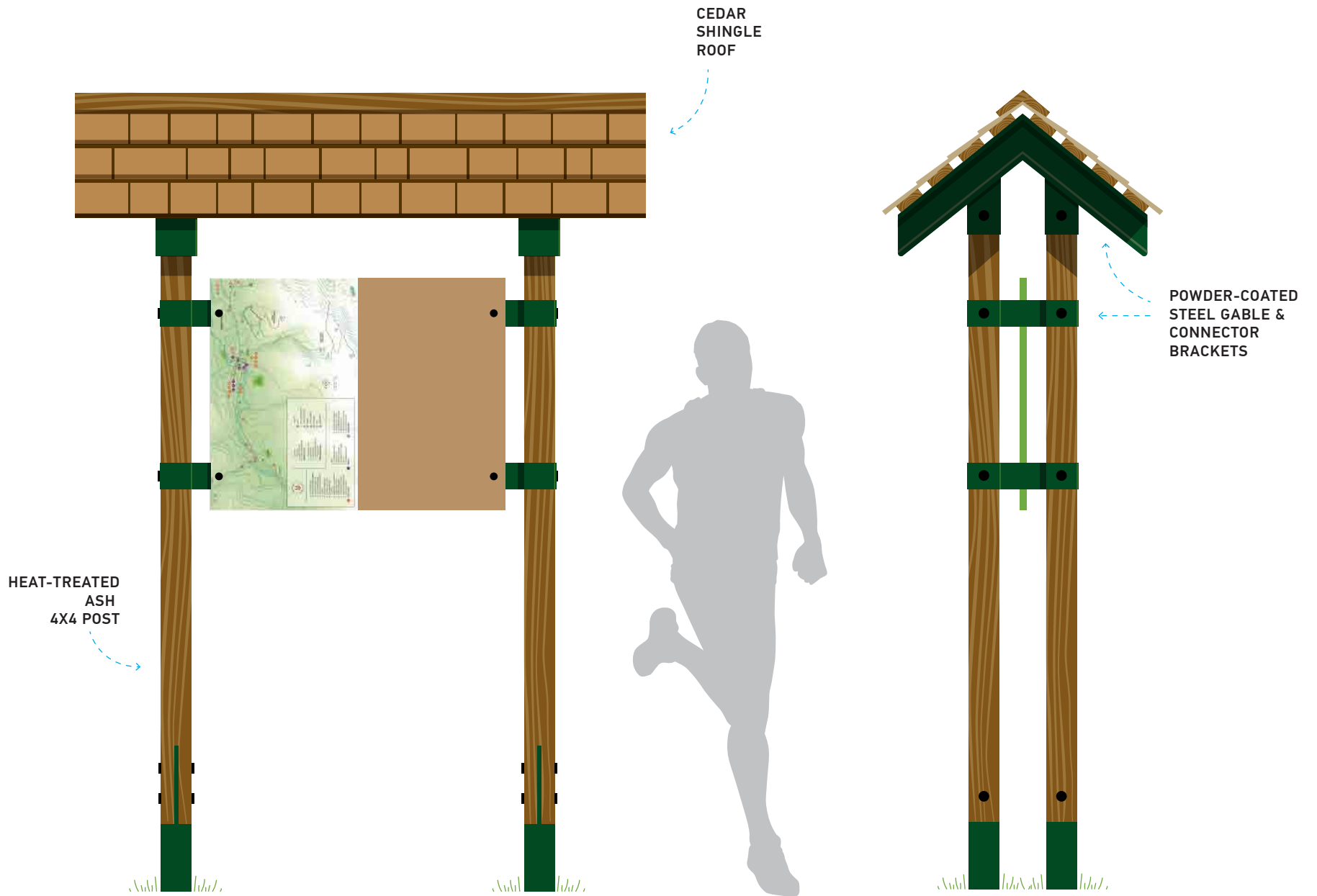
TRAILHEAD KIOSK SIGN (OPTION A)
